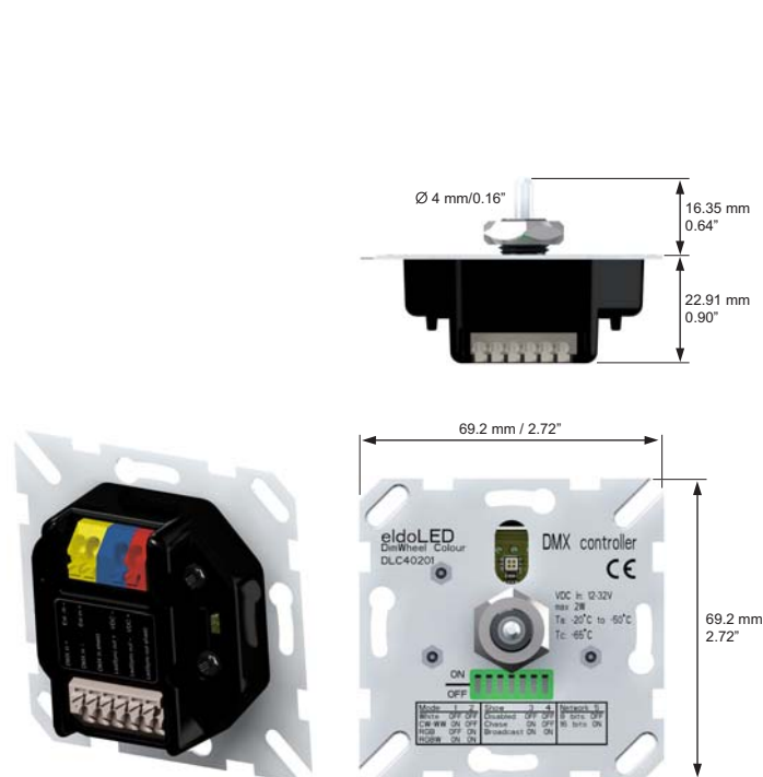
DimWheel Colour EU/UK dimensions (DLC40201)
