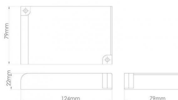
SENSE 1050mA /4000lm DRIVER DALI
