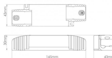
SENSE 1050mA /4000lm DRIVER NON DIM
