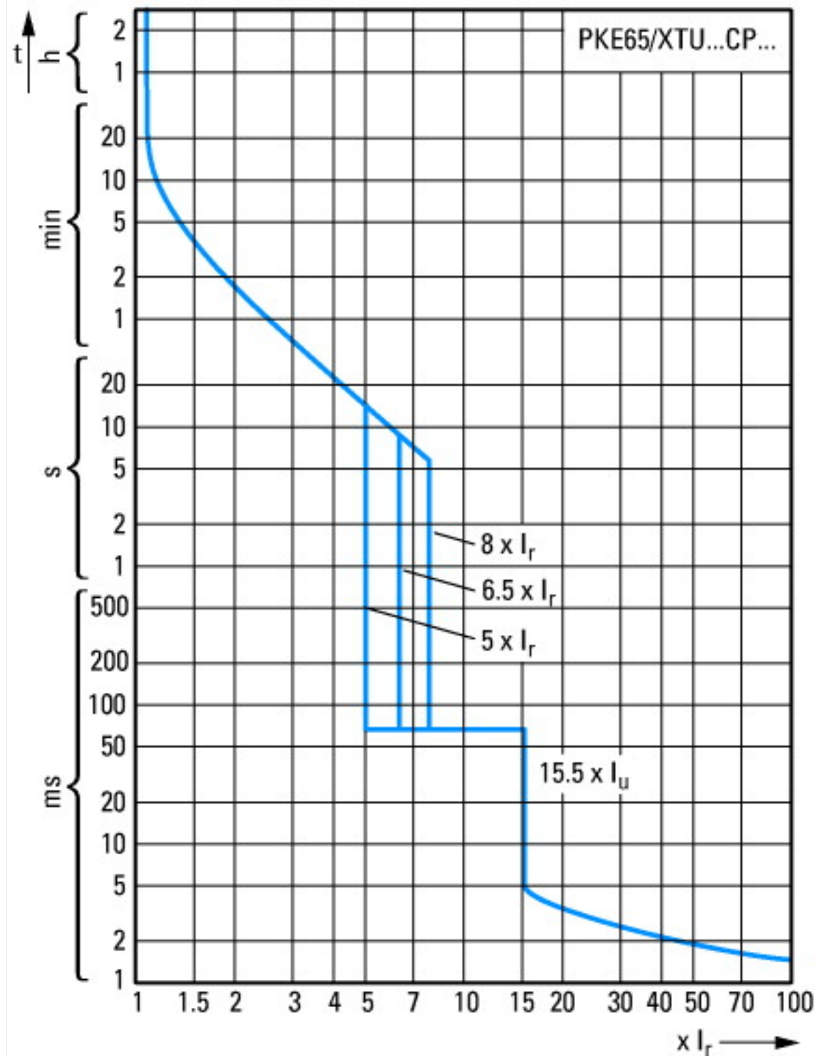
Tripping characteristics
