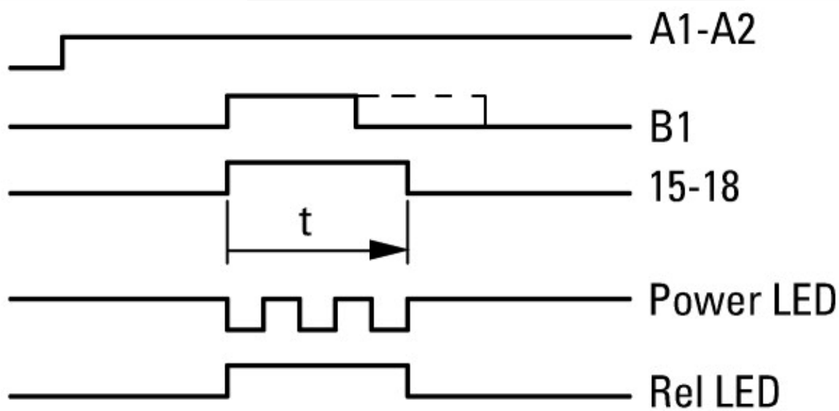
82 Pulse shaping
