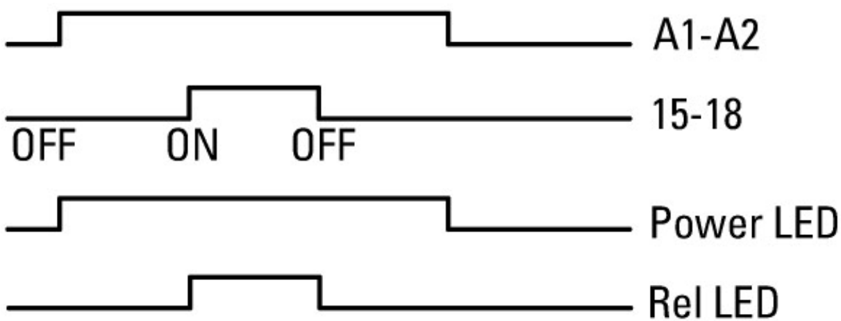
On-Off function
