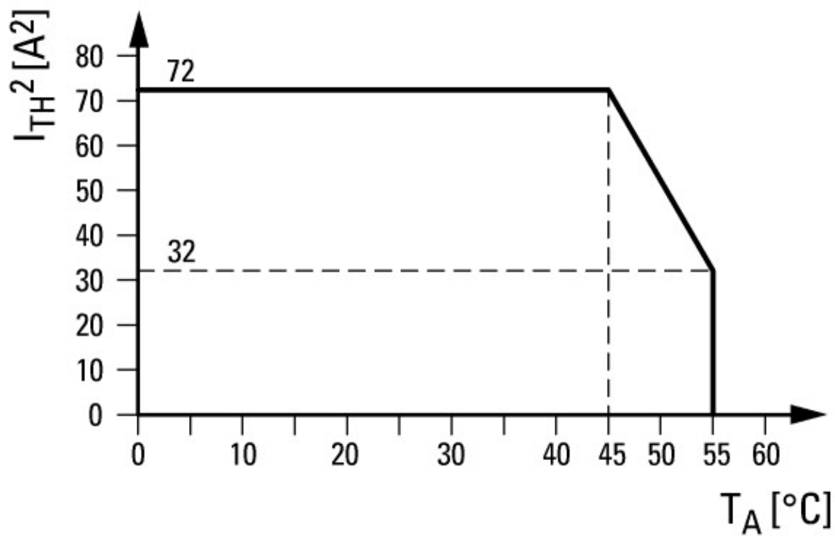
Derating curve
