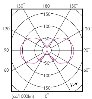
LEDBulb CLA 8-60W E27 G93 Clear 827 DIM
