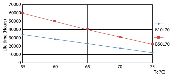
TLED_220-240V_G13-LifetimeVsTc
