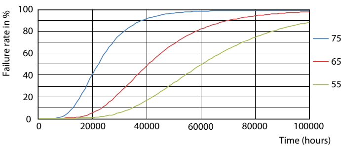
TLED_220-240V_G13-FailureRate
