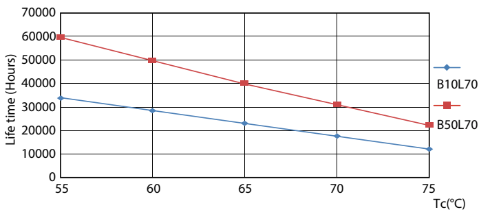
TLED_220-240V_G13-LifetimeVsTc
