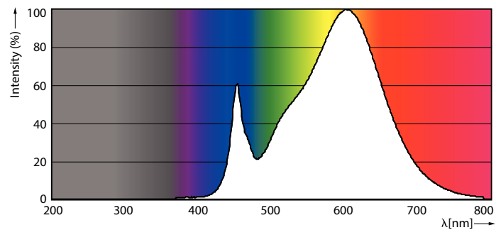
TLED_4ft_220-240V15.5-36W_2300lm_3000K_G13
