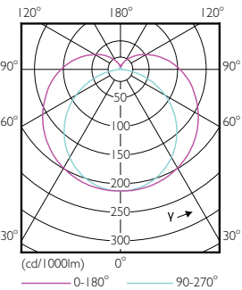
LEDtube 900mm 8-5W G13 833 750lm T8
