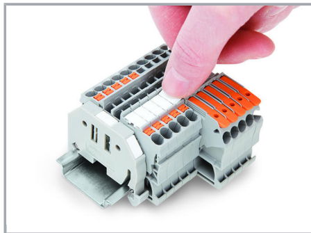
Snapping a marking strip into the marker slot. Snapping a marking strip into the marker slot.
