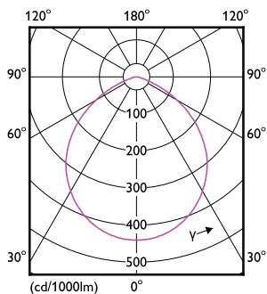
Downlight DN060B LED18S 840 PSU WH
