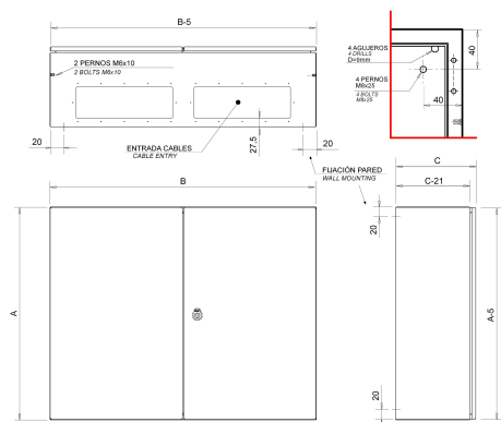
Standard drawing
