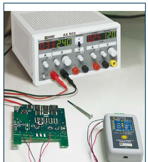
L432 recording two DC voltage supplies.
