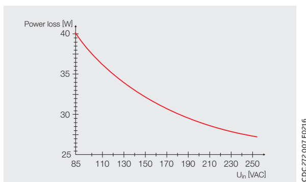
Typical power loss over AC input voltage
