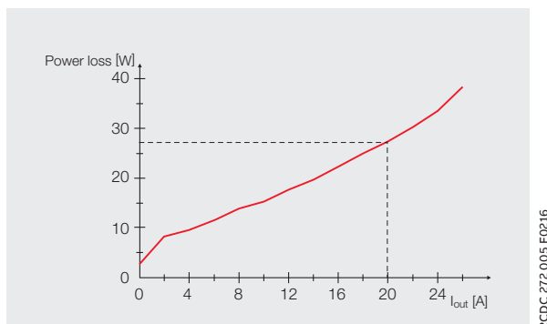
Typical power loss over output current
