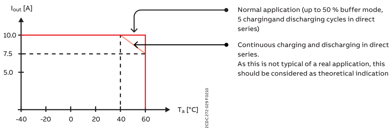
Characteristic curve of the temperature at rated load
