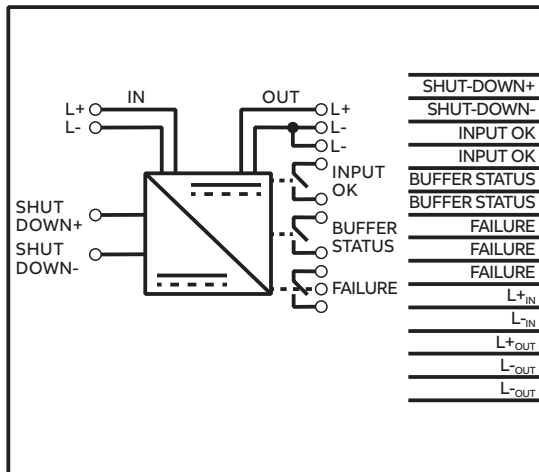
Connection diagram
