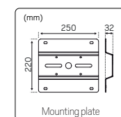
Mounting plate
