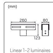
Linear 1-2 luminaires
