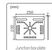
Junction box plate
