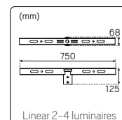
Linear 2-4 luminaires
