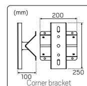
Corner bracket
